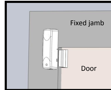
Right hand door mounting (arrow pointing down, magnet on right side)
